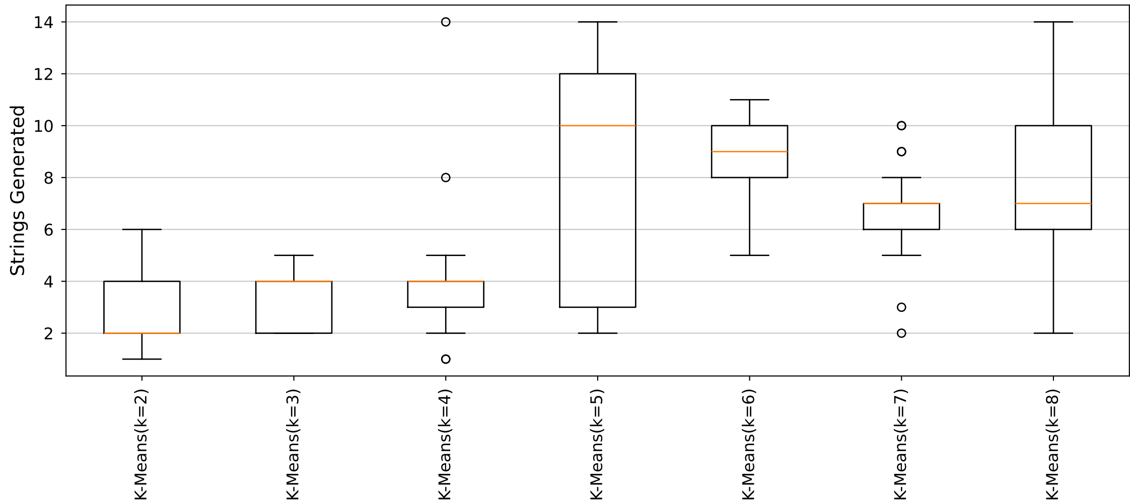
YARA Rules Strings Generated Distribution (Cluster16_Size8 dataset)
